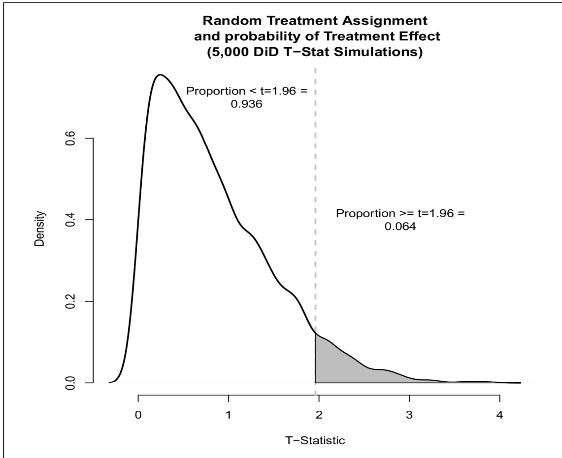
Figure 5. T -statistic random assignment simulations. Note. DiD = difference in difference.
